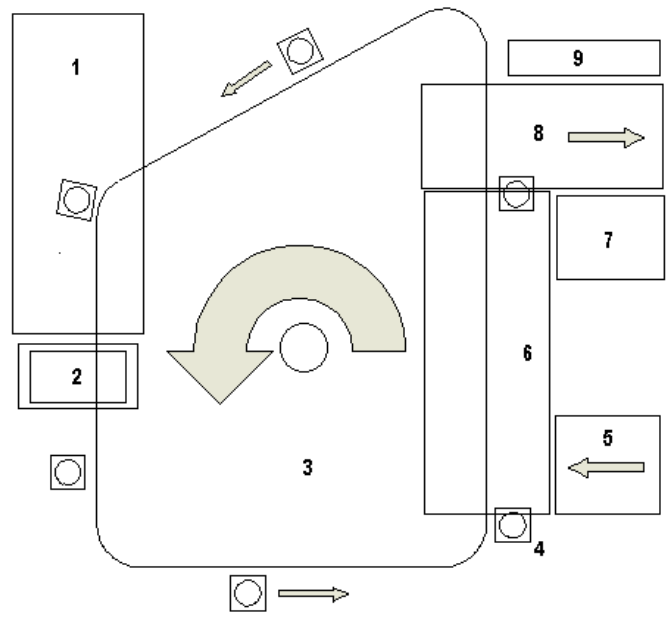
Fig.4 Layout of the Machine
