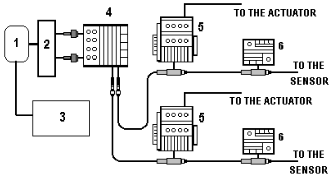
Fig.5 Network arrangement for the control
